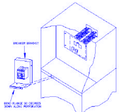
Fig. 3 HB3000 - HB6000 HEATER INSTALLATION
