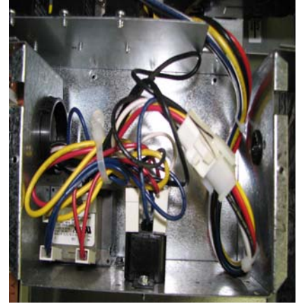
FIG. 2 – Connected (6) pin socket.
