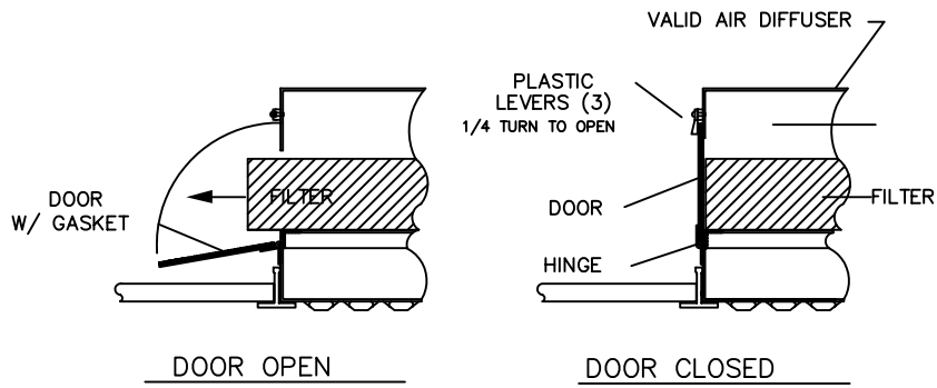
RIGHT SIDE VIEW - DETAILS
